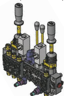
Dual levers with on-off FRV 60/8-E
